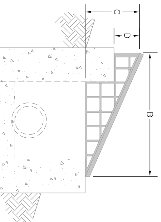
SECTION
